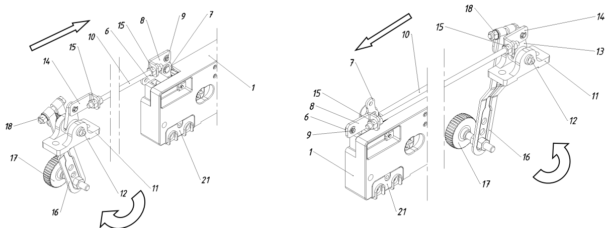
FIGURE 3 (PUSH OPERATION)
