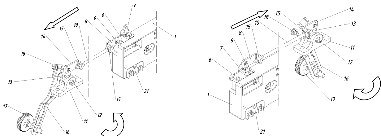
FIGURE 2 (PULL OPERATION)
